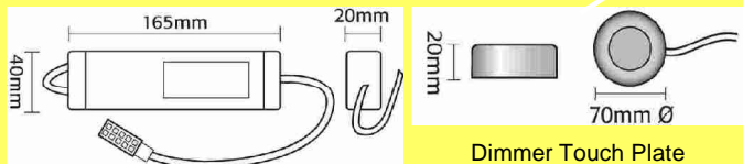
Dimmer Touch Plate
